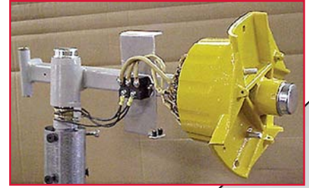
Rotor, stator, diode rectifier, slip rings, and bearings exposed on a Bergey XL.1 1 KW generator.
